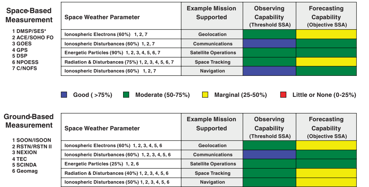
Figure 9. Sources and types of space weather data needed to support representative military mission areas. Color coding indicates the Air Force Weather Agency’s current capability level. (Image courtesy of Herbert Keyser, U.S. Air Force.)
